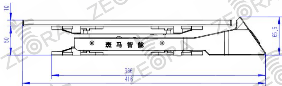
Overall Structure of the Intelligent Weighing Module
